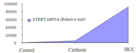
Fig. 7: hTERT mRNA (Relative unit) among the three studied groups
