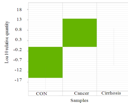
Fig. 9: Gene expression levels of hTERT mRNA for both control and HCC relative to cirrhosis
